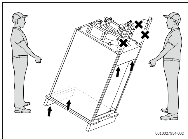
Sl.49 Transport boilerja
